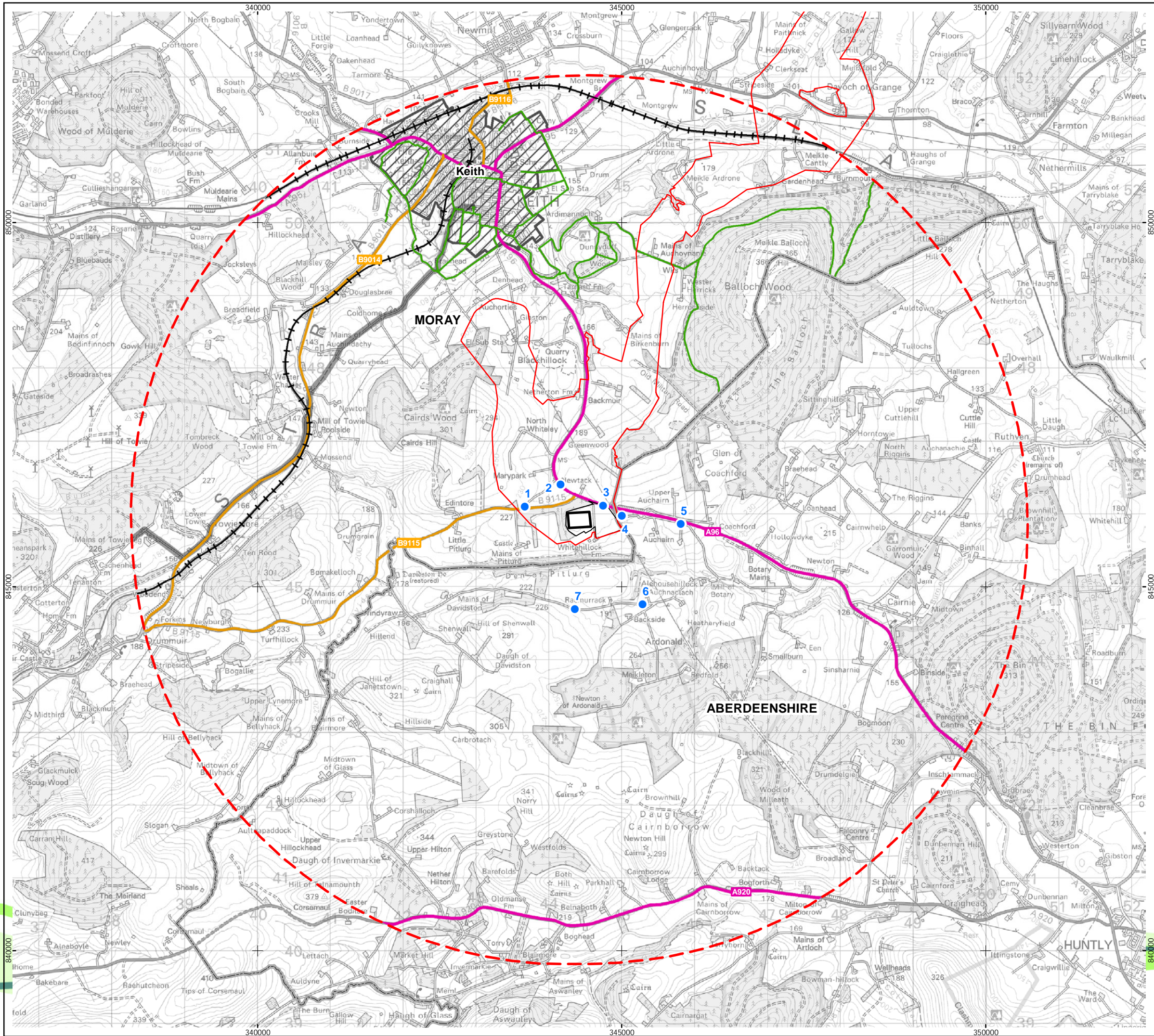
Figure 7.3.8 OnTI Onshore Substation Visual Receptors / Viewpoint Locations
