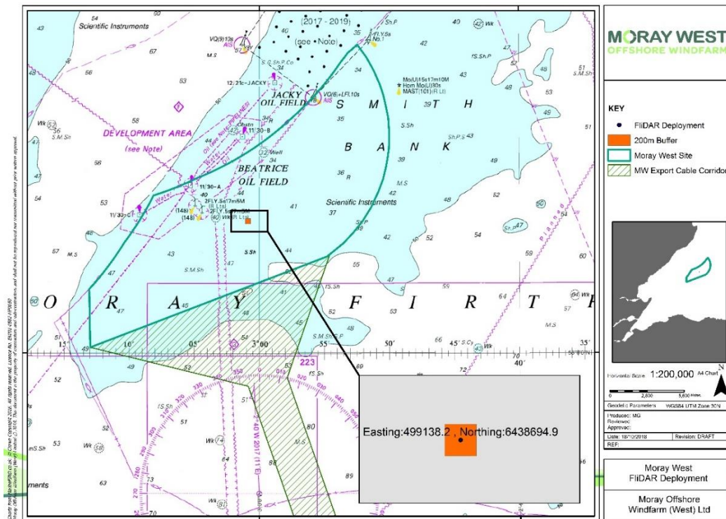
Floating LiDAR Buoy Location
